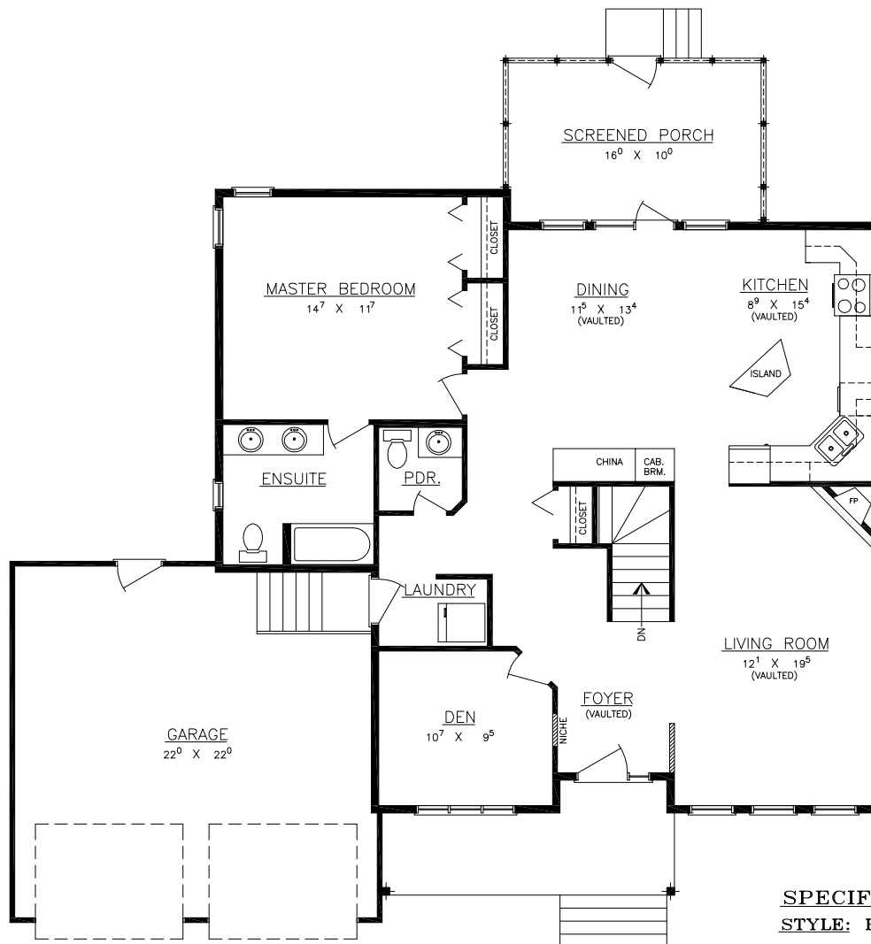
FLOOR PLAN
